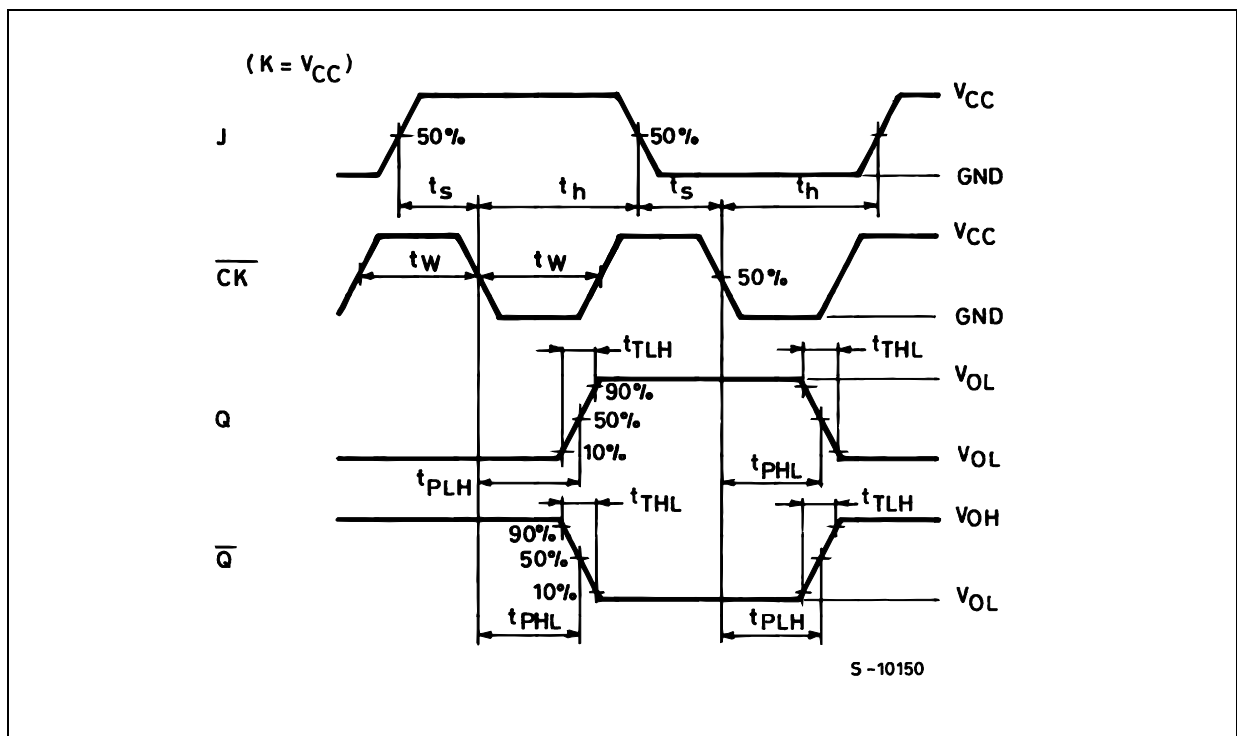
WAVEFORM 3 : PROPAGATION DELAY TIME, MINIMUM PULSE WIDTH, SETUP AND HOLD TIME ( f=1\text{MHz} ; 50% duty cycle)
