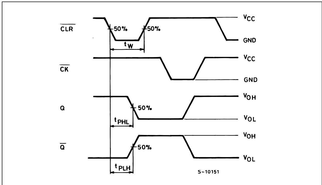
WAVEFORM 3 : PROPAGATION DELAY TIME, MINIMUM PULSE WIDTH, SETUP AND HOLD TIME ( f=1\text{MHz} ; 50% duty cycle)
